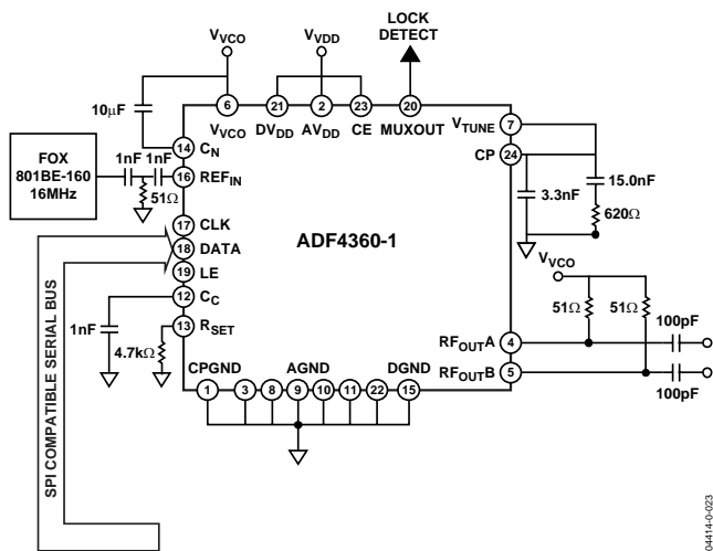
Figure 16. Fixed Frequency LO
